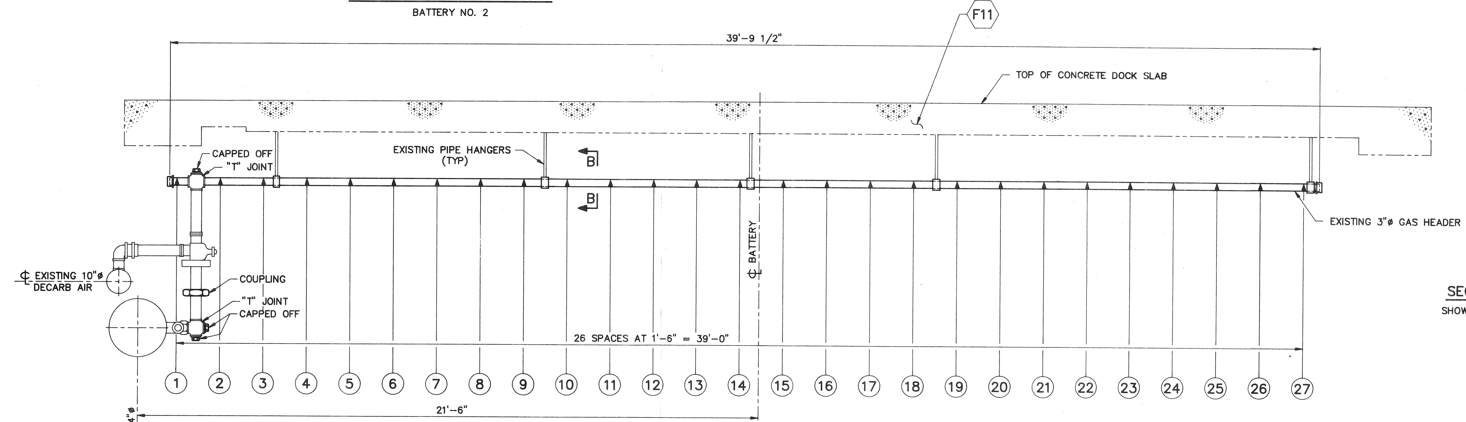
SECTION "A-A" (LOOKING SOUTH) TYPICAL SECTION OF 3" DIA. LONG GAS HEADERS (A DENOTES LOCATIONS OF ULTRASONIC THICKNESS TESTING)
